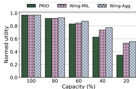
Figure 10: Benefits of Wing guidance. This figure shows the value attained for each scheduling policy, normalized to total value achievable. Wing-guidance (exemplified in Wing-Agg and Wing-MIL) is significantly beneficial at constrained capacities.
