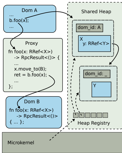
Figure 2: Inter-domain communication. Domain A invokes method foo() of domain B. The proxy that interposes on the invocation moves the ownership of the object pointed by x between domains.
