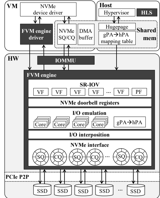
Figure 7: FVM architecture
