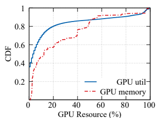
Figure 1: GPU resource statistic on a GPU production cluster.
