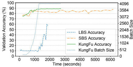
Fig. 4: Adaptive batch size (ResNet-56)
