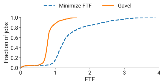
(b) CDF of finish time fairness metric (input job rate = 2.6 jobs/hr).
