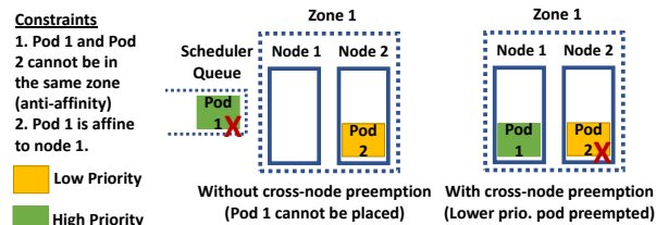
Figure 3: An anti-affinity constraint prevents Pod 1 and Pod 2 from being in the same zone, pod 1 is affine to node 1, and pod 2 has a lower priority than pod 1. Placing pod 1 on node 1 requires evicting pod 2 on node 2.
