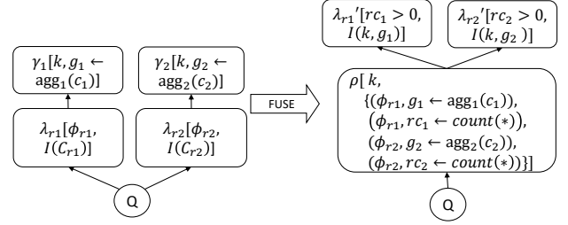
Figure 12: GROUPBY query fusion. Both rc_1 and rc_2 are fresh column names.
