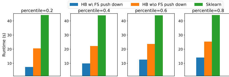
Figure 9: Feature selection push down.
