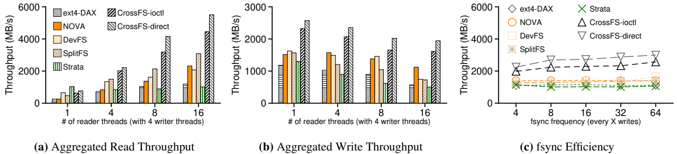
Figure 3: Microbenchmark. Throughput of concurrent readers and 4 writers sharing a 12GB file. For CrossFS and DevFS, 4 device-CPU are used. CrossFS-iocctl uses IOCTL commands bypassing VFS but with OS traps, whereas CrossFS-direct avoids OS traps and VFS. Figure 3a and Figure 3b are random accesses. Figure 3c shows the impact on performance when varying the commit frequency with 4 concurrent writers.
