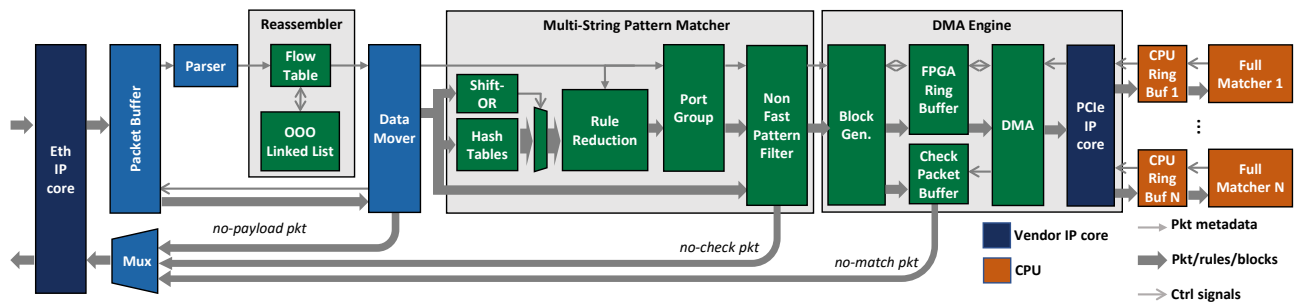
Figure 4: Pigasus architecture.
