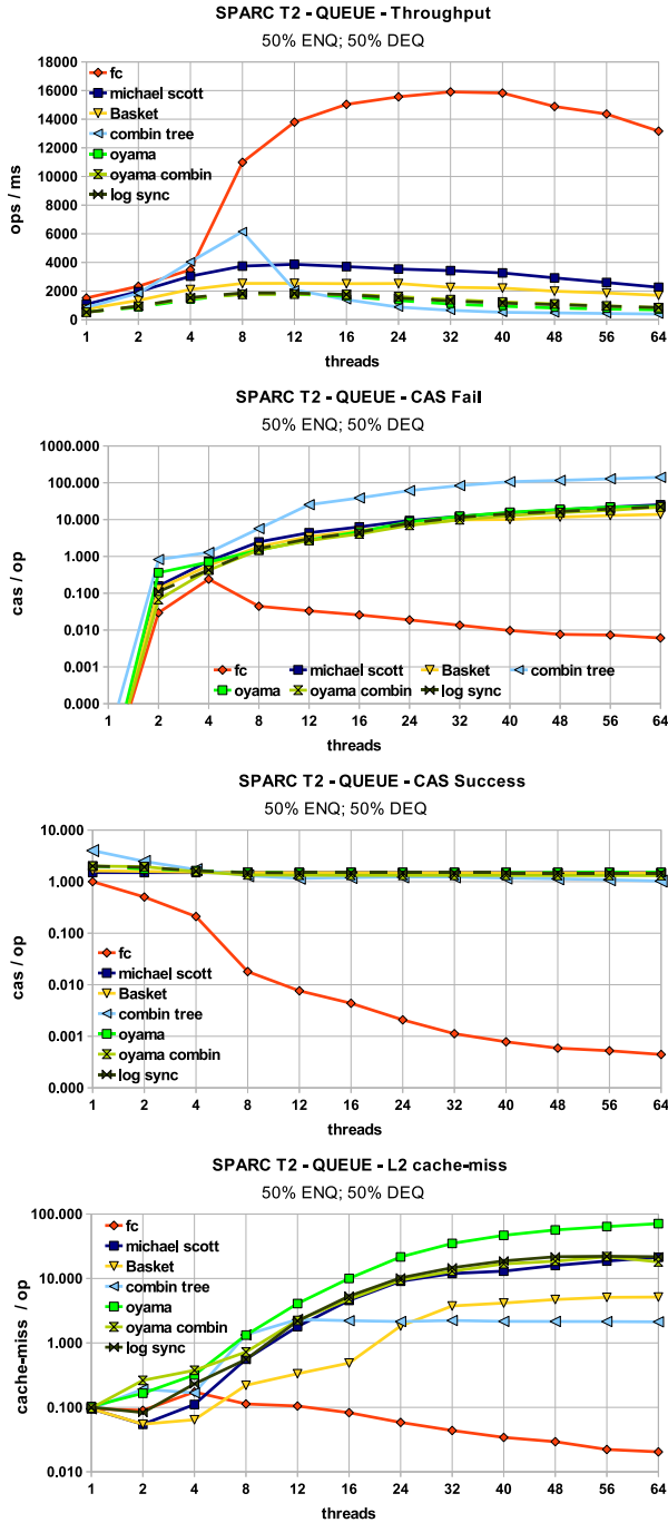
Figure 2: Concurrent FIFO Queue implementations: throughput (number of operations), average CAS failures (per operation), average CAS successes (per operation), and L2 cache misses (per operation).
