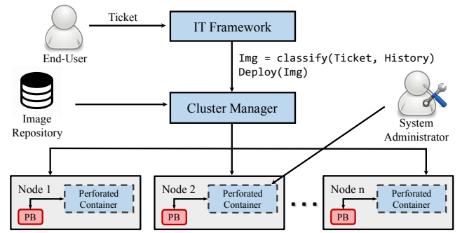
Figure 3: WatchIT architecture overview. PB is the permission broker.
