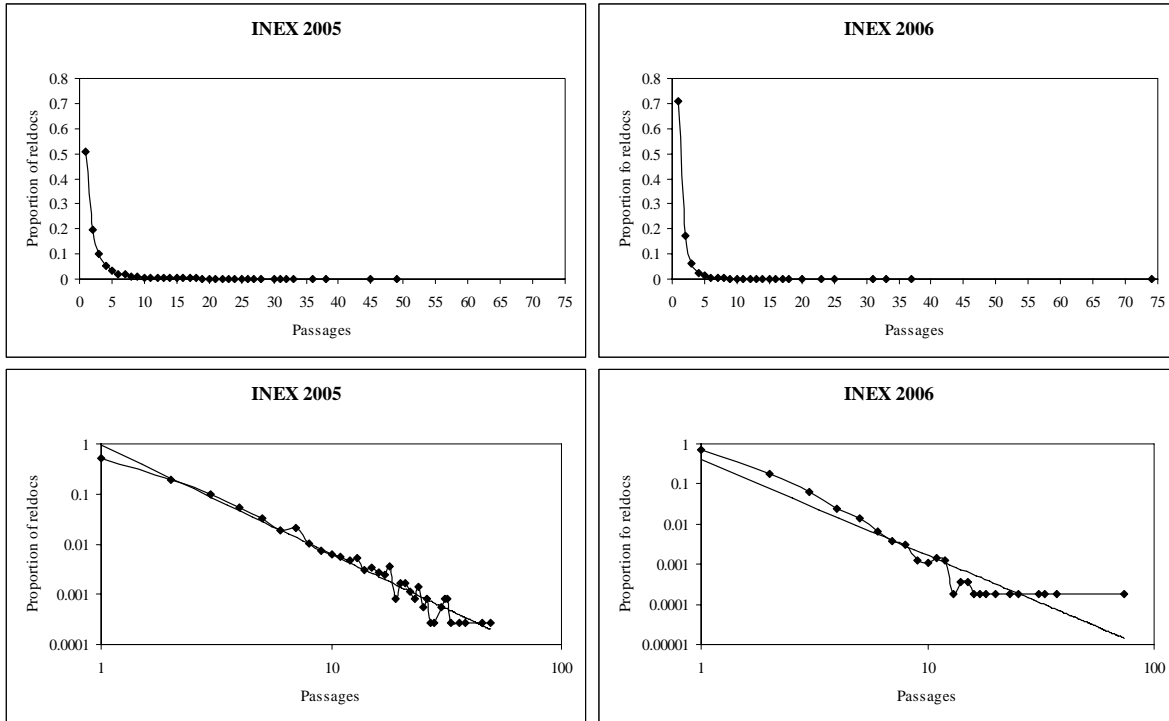
Figure 6: Proportion of relevant documents containing the given number of relevant passages. Linear scale (top) and log-log scale (bottom). The distribution is approximately power law (shown). Highlighting was not used prior to 2005.
