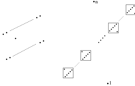
Figure 1: Indecomposable permutations in av(2413, \mathcal{IW}) and av(3142, \mathcal{IW})
