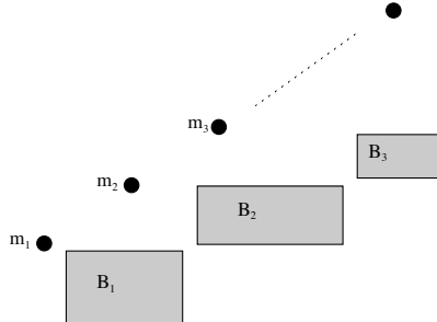
Figure 2: Structure of a permutation in av(2431, \mathcal{IW})
