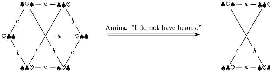
Figure 7: In the epistemic state (Hexa, \clubsuit\heartsuit\spadesuit) Amina announces that she does not have hearts.
