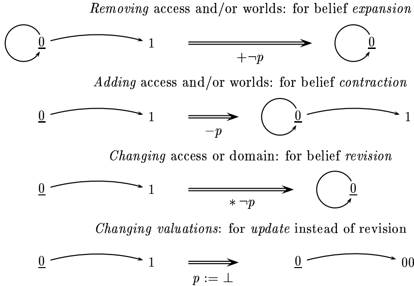
Figure 13: Possible changes of belief mirrored in Kripke structure transitions
