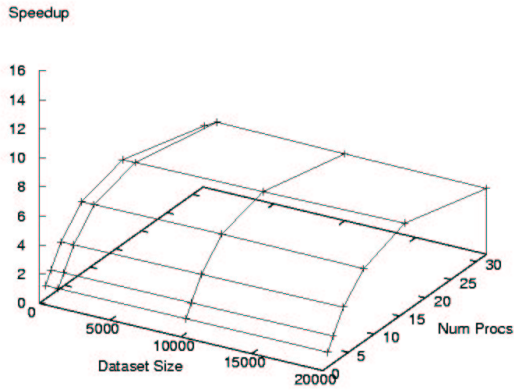
Figure 3. Speedup of Node Parallel as the data set size increases (Network Size 2,000)
