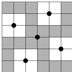
Figure 1: A permutation in \text{Av}(1324, 4231) containing 41352.
