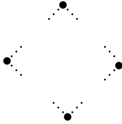
Figure 3: The form of a simple permutation not containing 41352 or 25314.
