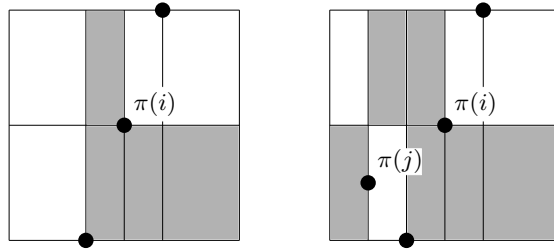
Figure 2: The situation in the proof of Proposition 3.
