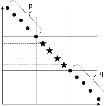
Figure 3: An irreducible permutation in \text{Av}(\alpha_r, \beta_{pq})
