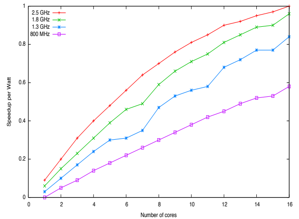
Figure 2. Speedup per Watt for raytrace
